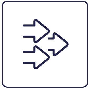
Iterative Workflow
