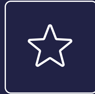
STAR Framework
